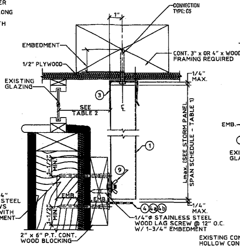
H CEILING/BUILD-OUT MOUNT SECTION SCALE: 3" = 1' - 0"
