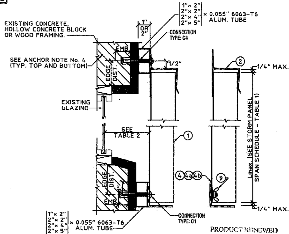
(P) WALL MOUNT SECTION SCALE: 3" = 1'-0"
