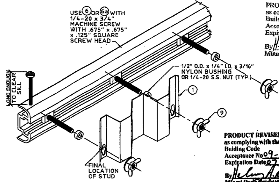
M C-TRACK ASSEMBLY (ISOMETRIC VIEW) N.T.S.
